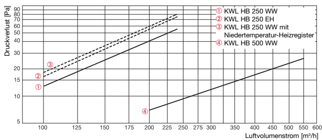
(Abb. Type KWL HB.. WW)
